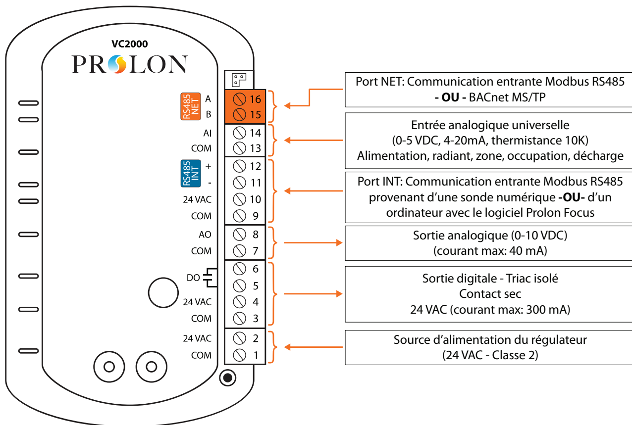
Figure 2 - Identification des borniers
