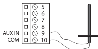
Figure 6 - Auxiliary Input
