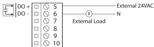
Figure 8 - Typical Wiring of Digital Output
