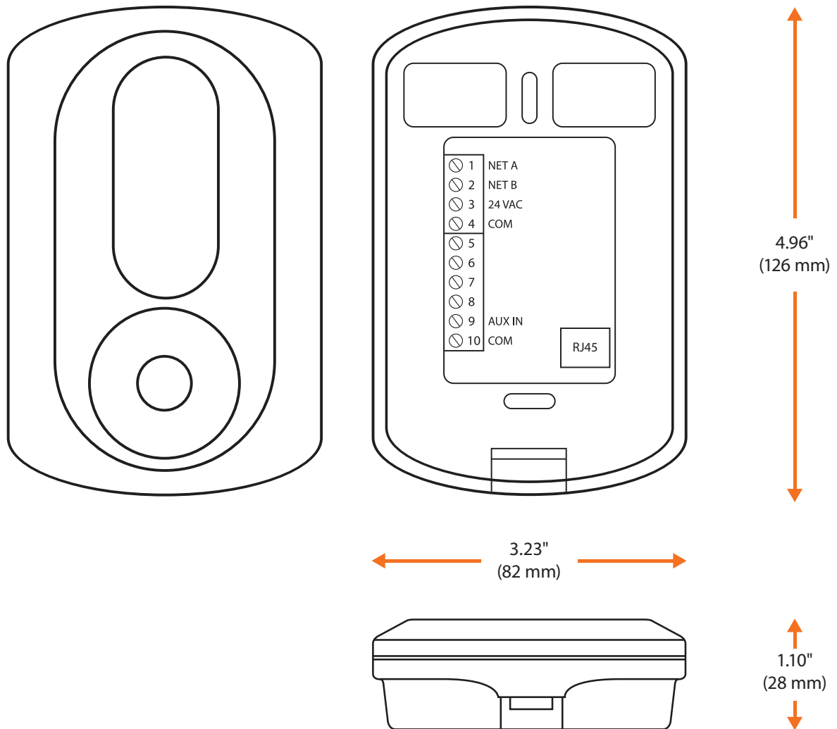
Figure 13 - T1100 Size Diagram
