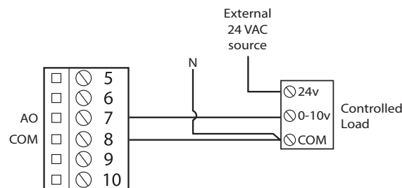
Figure 9 - Typical Wiring of Analog Output
