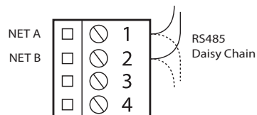
Figure 4 - Network Connection
