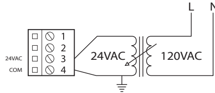
Figure 3 - Power Source
