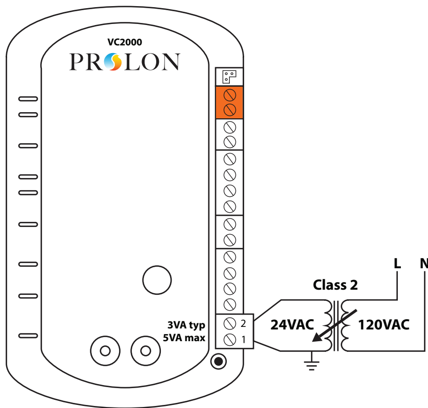
Figure 4 - Power Source
