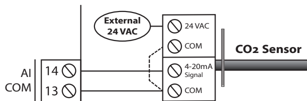
Figure 7 - CO 2 Sensor
