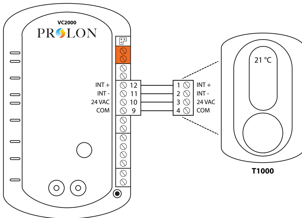
Figure 18 - Interface Port
