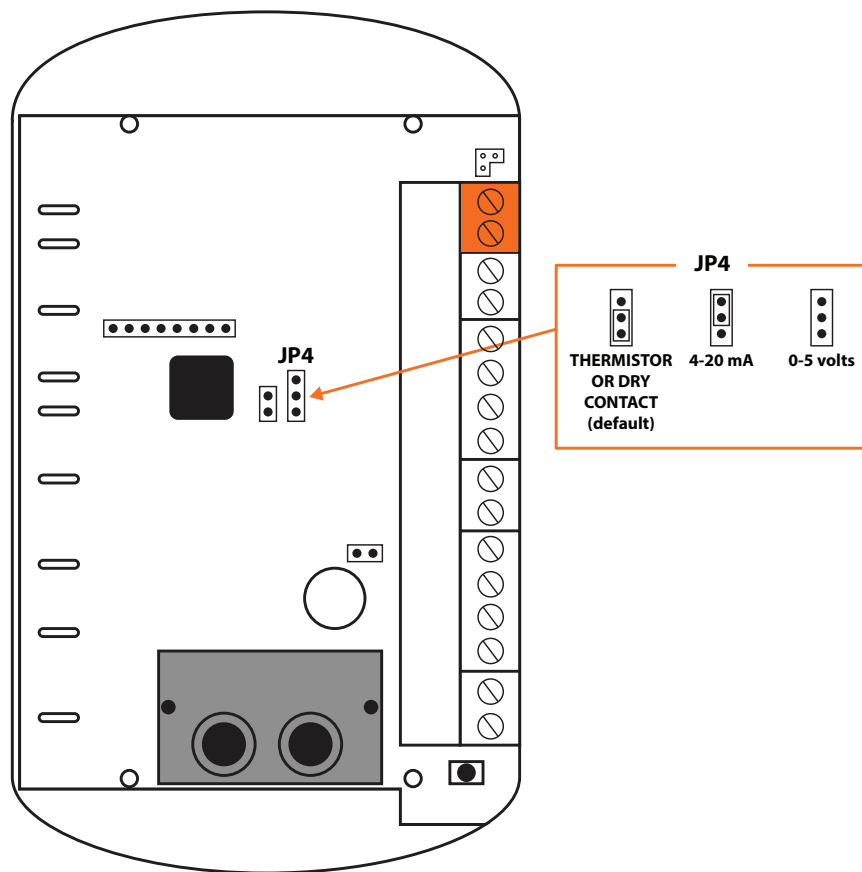
Figure 5 - Analog Input
