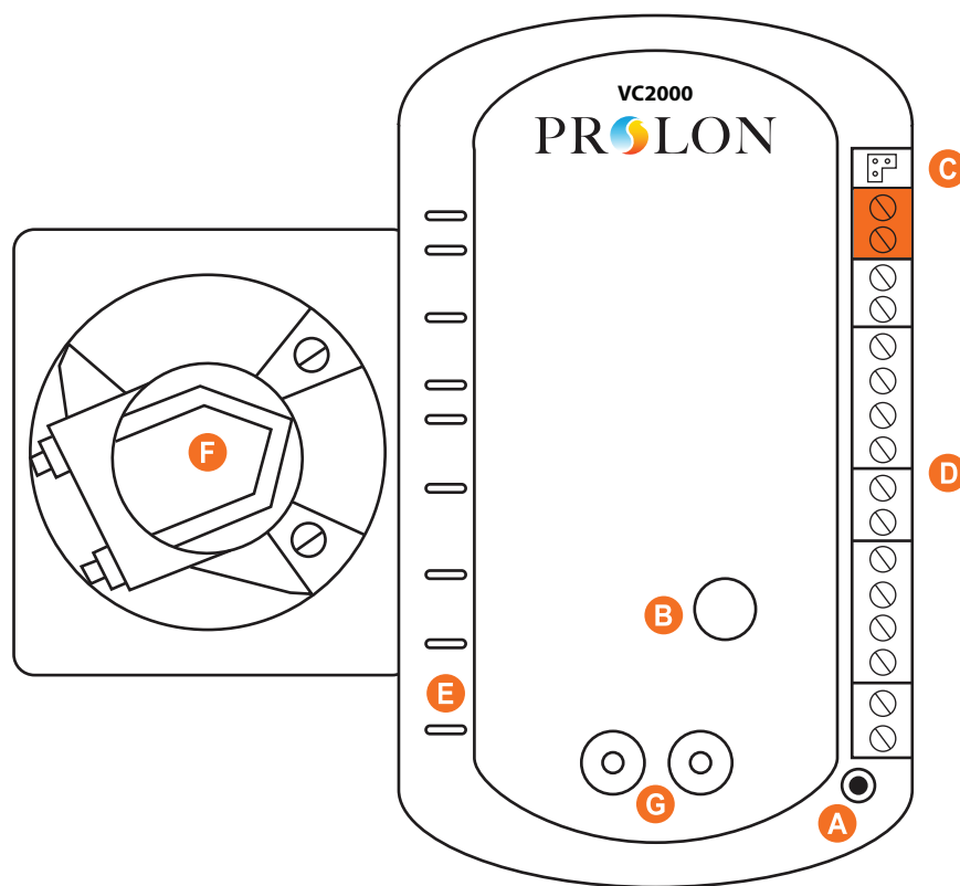
Figure 1 - Component Identification
