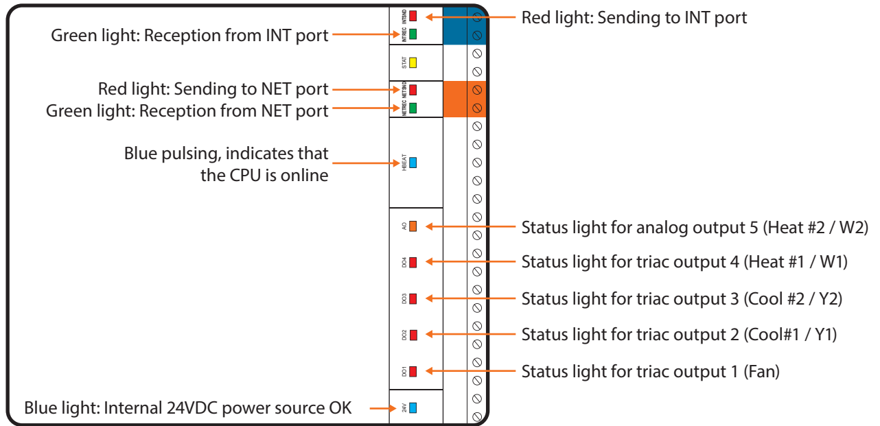
Figure 2 - LEDs Identification
