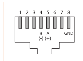
Figure 8 - Raccordement RJ45
