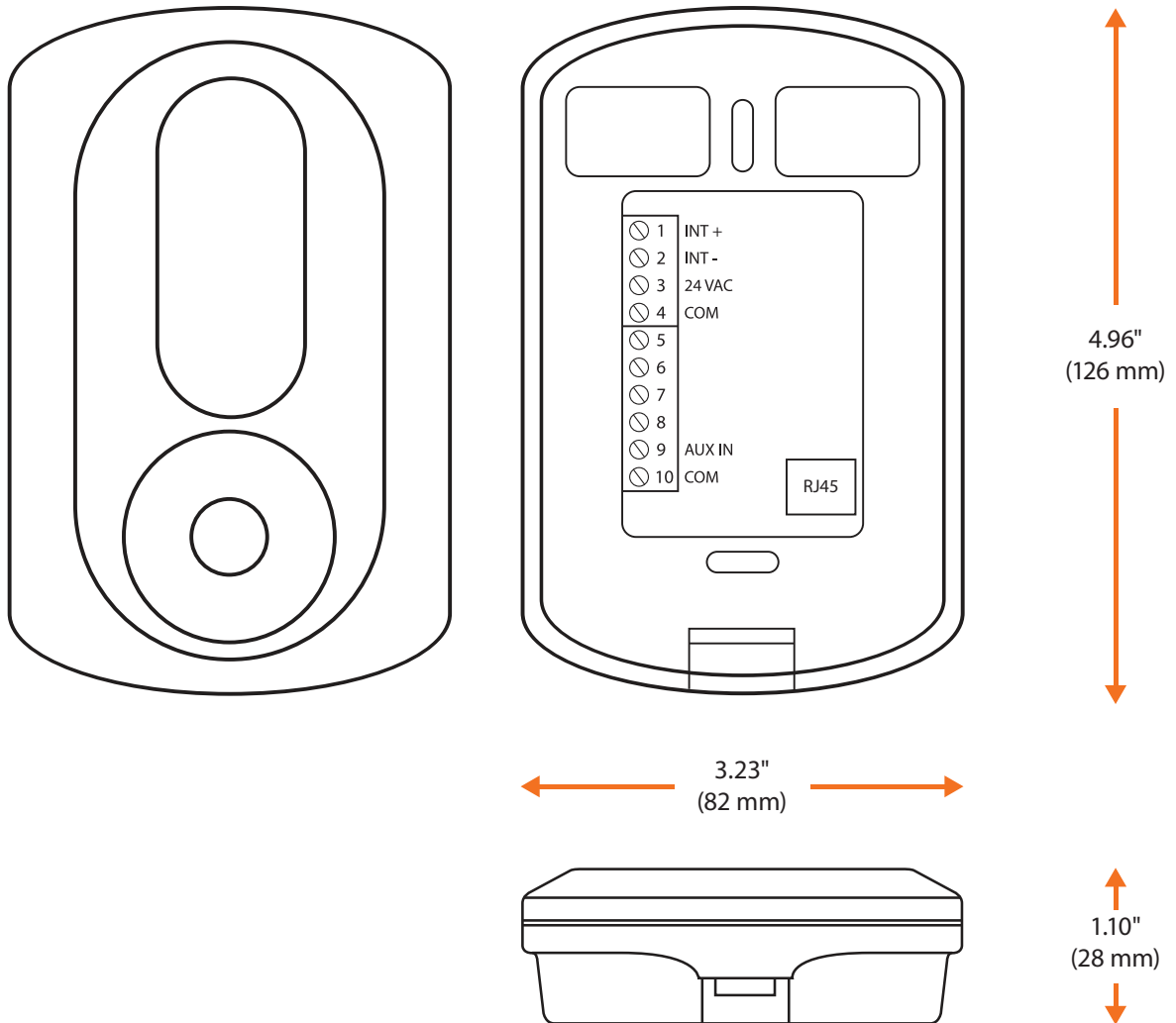
Figure 11 - T1000 Size Diagram
