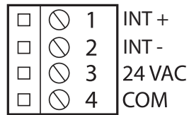
Figure 3 - Terminal Block
