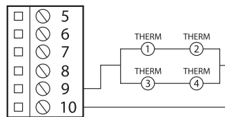
Figure 6 - Averaging multiple remote sensors (Series-Parallel)
