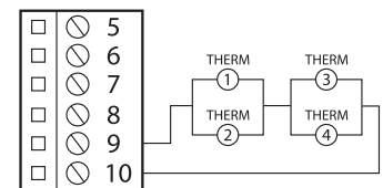
Figure 7 - Averaging multiple remote sensors (Parallel-Series)
