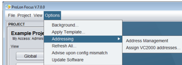
Figure 50 - Addressing Menu
