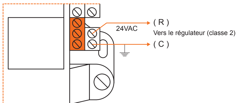
Figure 31 - Raccordement de l'alimentation 24 VAC
