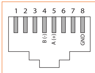
Figure 25 - Raccordement RJ45
