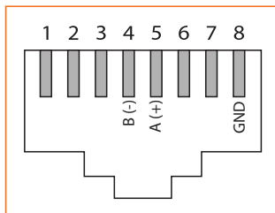
Figure 13 - Raccordement RJ45
