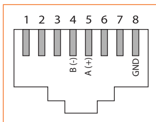
Figure 19 - Raccordement RJ45
