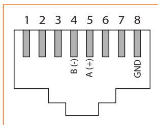
Figure 22 - Raccordement RJ45
