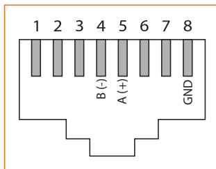
Figure 16 - Raccordement RJ45
