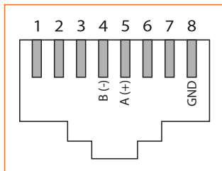
Figure 10 - Raccordement RJ45
