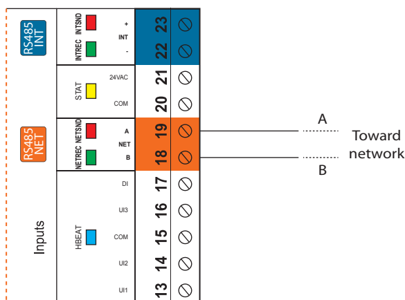
Figure 15 - Connecting to the Network
