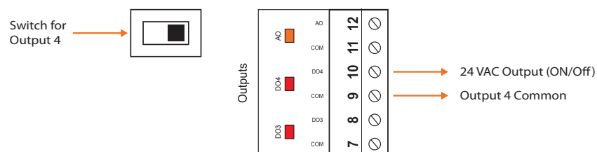
Figure 8 - Output in SOURCE mode
