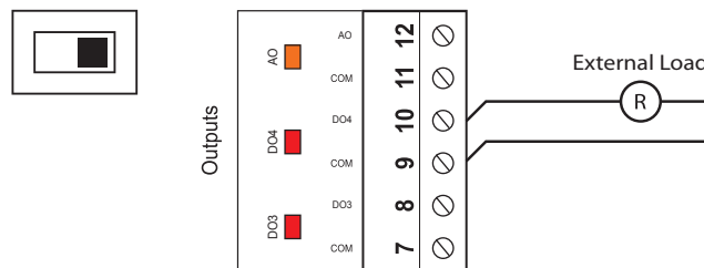
Figure 10 - Connection of Active Outputs 3 and 4
