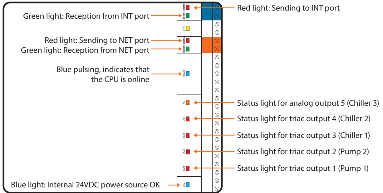
Figure 2 - LEDs Identification
