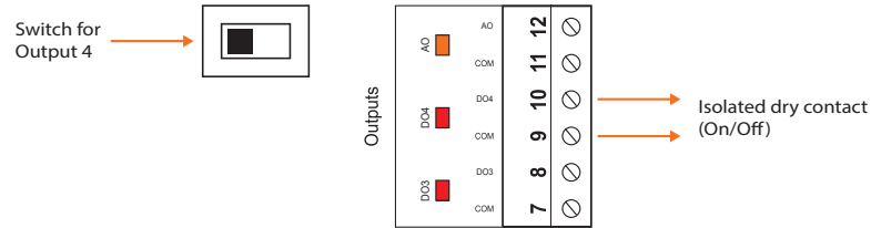
Figure 9 - Output in SINK mode
