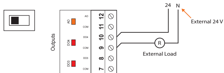
Figure 11 - Connection of Passive Output 3 and 4
