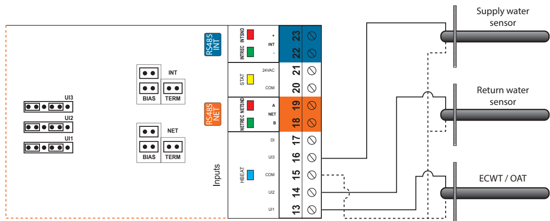
Figure 6 - Connecting the Temperature Sensors
