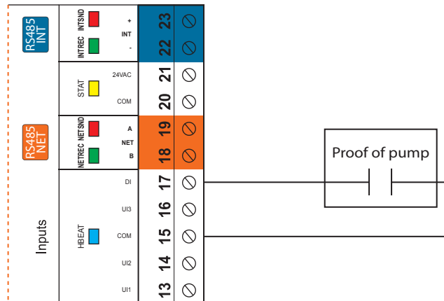
Figure 7 - Connecting the Proof of Pump Contacts to the Controller
