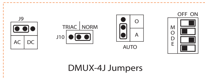
Figure 11 - Connecting the DMUX-4J (Powered by C1050)
