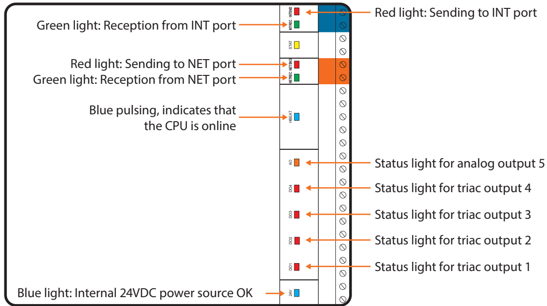
Figure 3 - LEDs Identification
