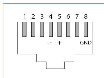
RJ45 Pinout
